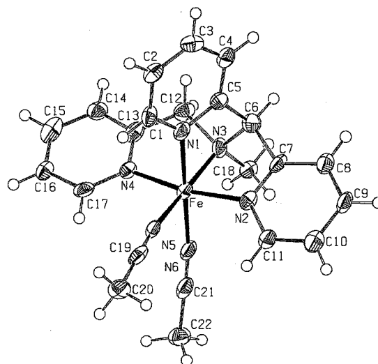
Figure 2. ORTEP plot of the cation of 4
