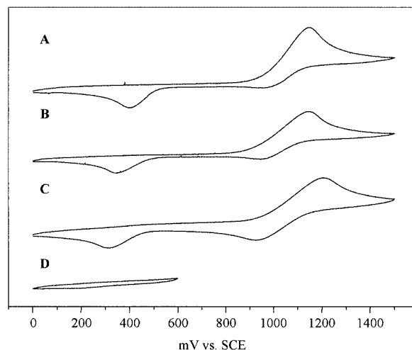
Figure 4. Cyclic voltammogram of 4 in acetone: (a) scan rate 50 \text{ mV/s} ; (b) Scan rate 100 \text{ mV/s} ; (c) scan rate 500 \text{ mV/s} ; (d) 600 \text{ mV} used as vertex potential
