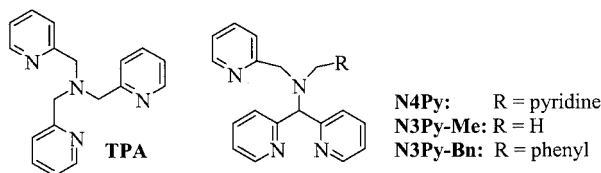
Figure 1. Ligands used for stereoselective epoxidation and cis -dihydroxylation of alkenes
