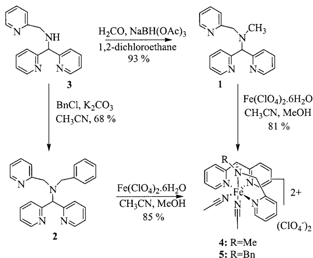
Scheme 1. Synthesis of ligands 1 and 2 and the corresponding iron(II) complexes 4 and 5
