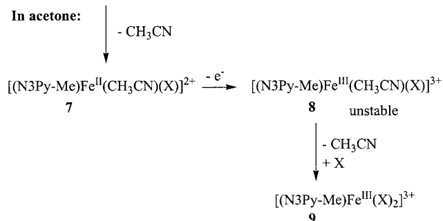
Scheme 2. Redox behavior of 4 in CH_3CN and acetone
