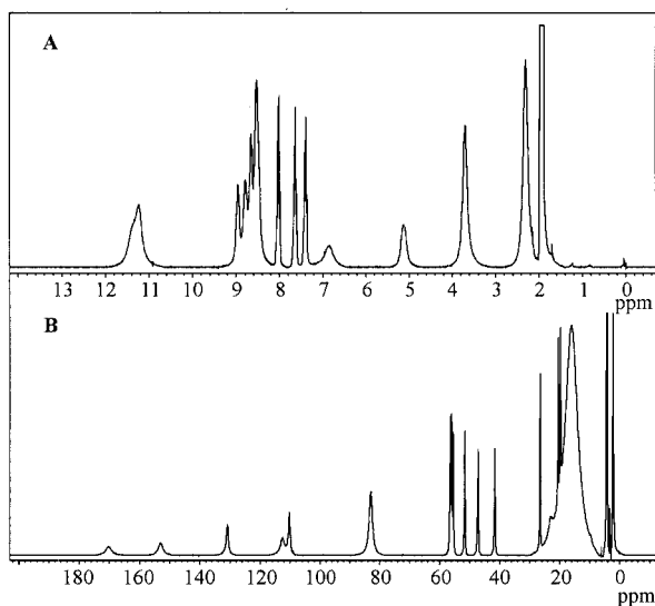
Figure 3. ^1\text{H} NMR spectrum of 4 (a) in CD_3CN and (b) in [D_6] acetone
