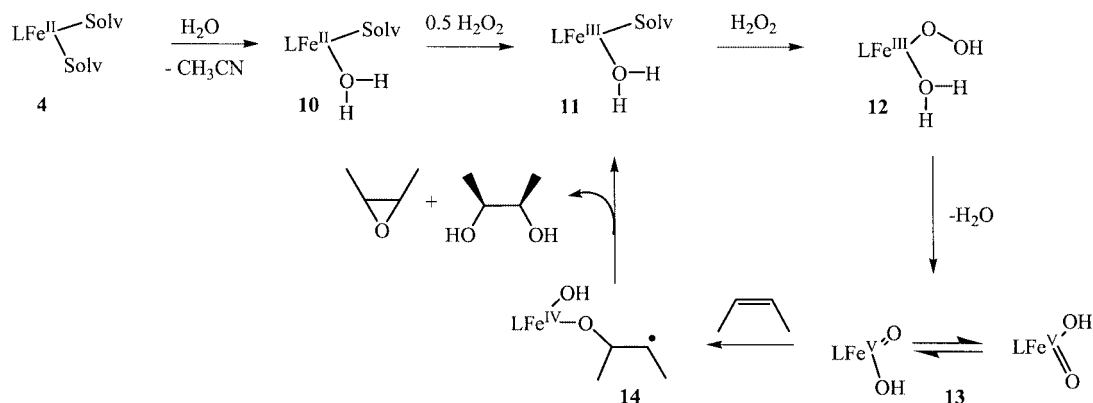
Scheme 3. Proposed mechanism for the catalytic oxidation by N3Py-MeFe(ClO 4 ) 2 (CH 3 CN) 2 in acetonitrile
