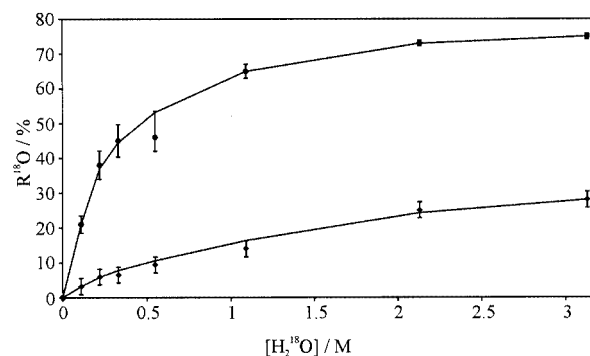
Figure 5. Incorporation of 18 O from H 2 18 O: • diol; ♦ epoxide
